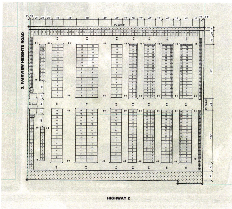
SCHEMATIC SITE PLAN #5 14810 W HIGHWAY 2 * MEDICAL LAKE, WA * 01.17.20
