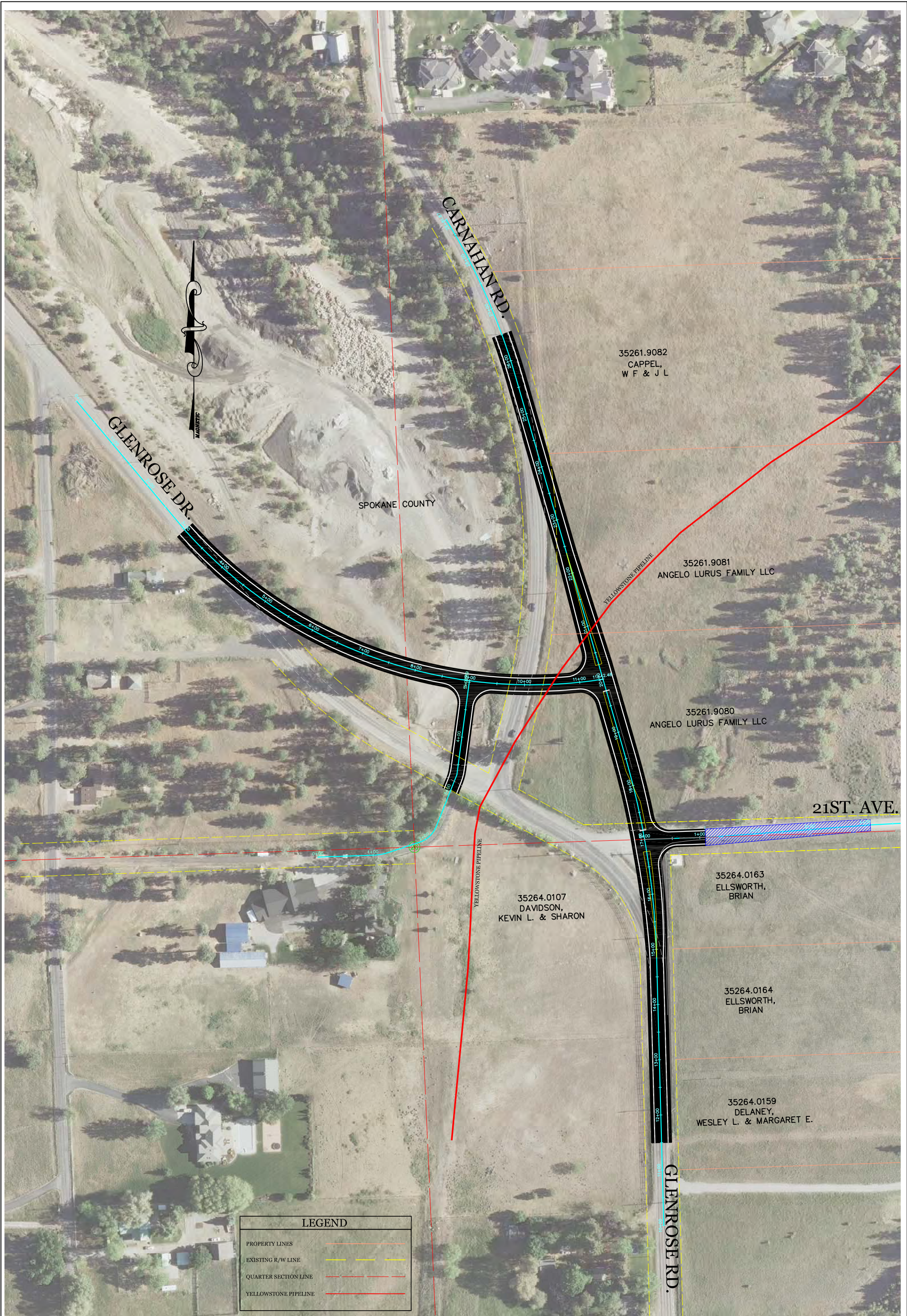
OPTION # 1 - CARNAHAN RD. / GLENROSE RD. - TEE INTRESECTION
